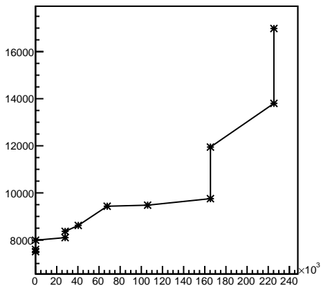
Maximum Busy time vs Event Number, usec
