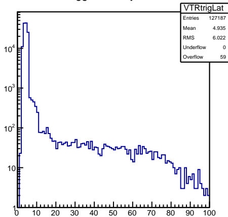
Trigger latency, usec
